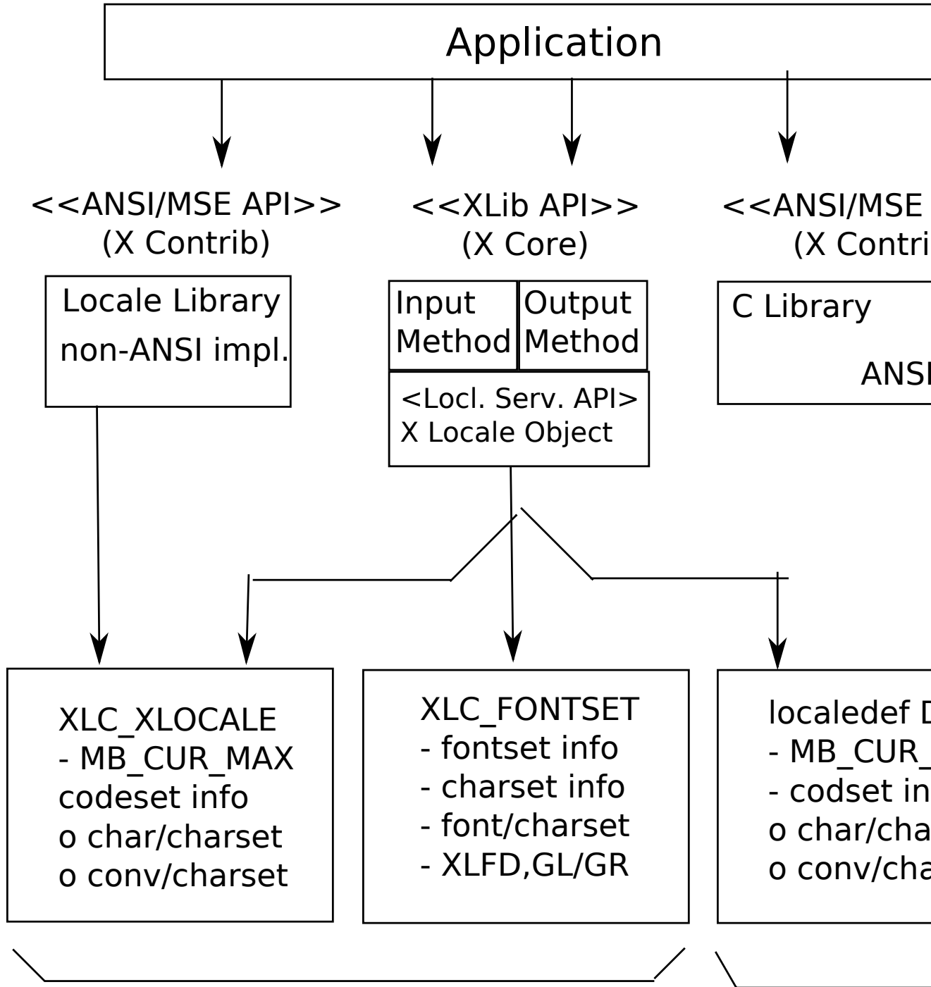
Frame work of Locale Service API Proposal
